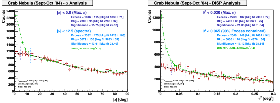
Figure 2. Crab Nebula \alpha -plot and \theta^2 -plot for SIZE > 180 phe. Two cuts applied: the one which maximize significance and the one which retain 99% of the excess signal. Results for ON-OFF f_{fit} are displayed in brackets.
