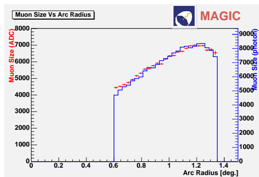
Figure 4. The dependence of SIZE_{muon} on R_{arc} is shown for data (red dots) and MC (blue histogram). After overall CE calibration good agreement is achieved.
