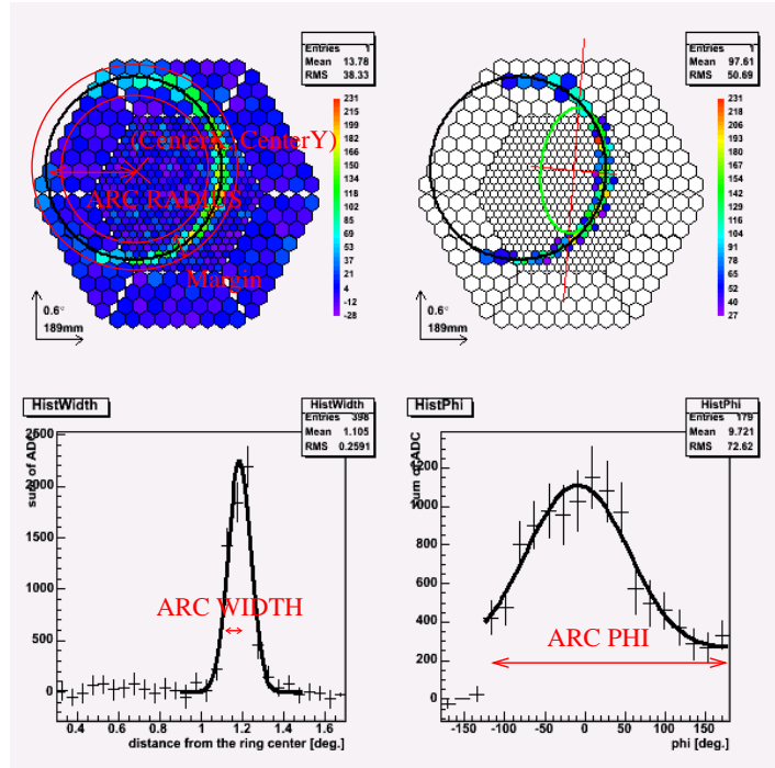
Figure 2. An example of a muon ring image in the MAGIC camera. The lower plots show the corresponding ARC WIDTH and ARC PHI distributions.
