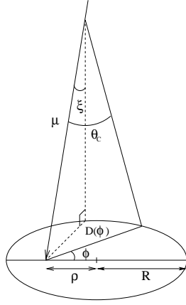
Figure 1. Geometry of Cherenkov light emitted by a muon hitting the reflector dish ( R : mirror radius, \rho : impact parameter, \xi : incident angle, \theta_C : Cherenkov angle
