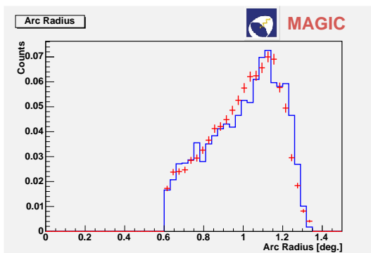
Figure 3. The distribution of the radius R_{arc} of the fitted muon rings is shown for data (red dots) and MC (blue histogram)
