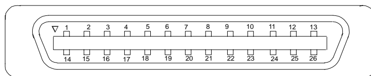
MDR 26 Position Plug ( Both Ends )
